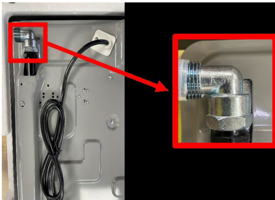
Figure 1 Gas inlet elbow original position on appliance
